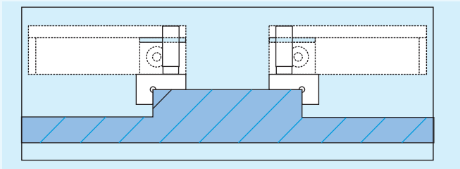
Shoulder Anvils Flat Outside Spigot Diameter
