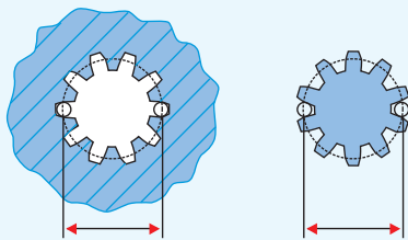
CYLINDRICAL MEASURING PINS FOR INTERNAL & EXTERNAL GEAR MEASUREMENT
