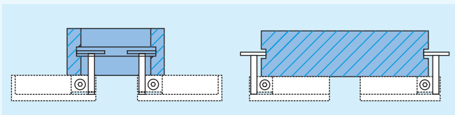
Disc Anvils For Measuring Groove Diameter
