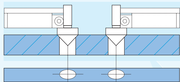
Cone Anvils For Measuring Hole Centre Distance
